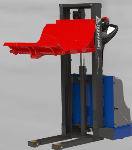
Fixed cradle with hydraulic lip
